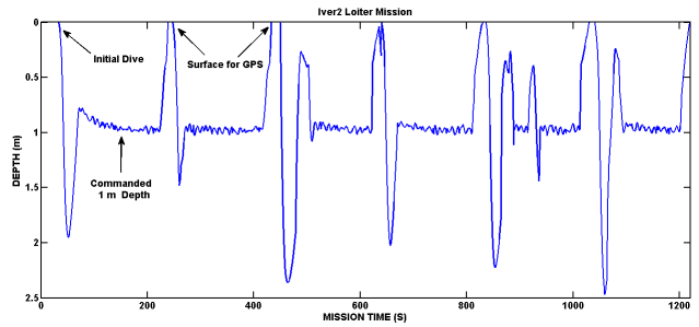
Fig. 6. A plot of the Iver2 depth during the hexagonal loiter backseat mission on the Charles River. As can be seen in the plot, the vehicle maintains its commanded one meter depth except when the periodic surface behavior forces the vehicle to surface for a GPS fix.
